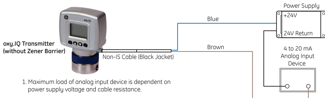
oxy.IQ Installation with Zener Barrier (top) and Installation without Zener Barrier (bottom)
